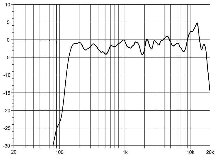
C4-TOP frequency response
