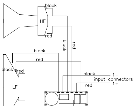
C4-TOP wiring diagram
