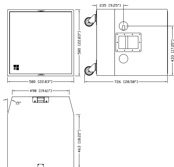
C4-TOP cabinet dimensions in mm [inch]
